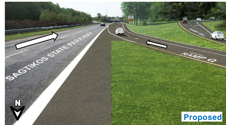
Ramps from eastbound and westbound LIE to southbound Sagtikos State Parkway and to Crooked Hill Road.
